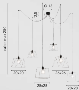
I-BROOKLYN-S6 8031440353748 6xE27
