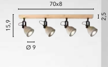
I-KISA-AP4 8031414897131 4xGU10
